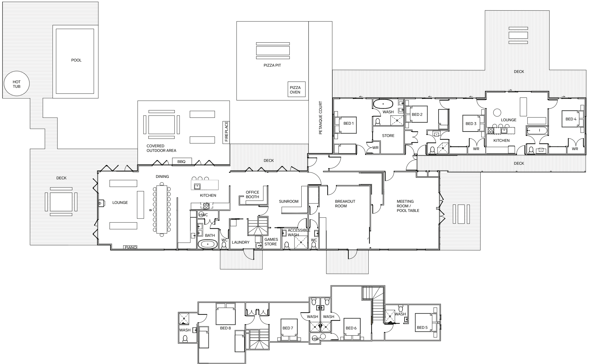
LAWN ROAD RETREAT FLOOR PLAN
